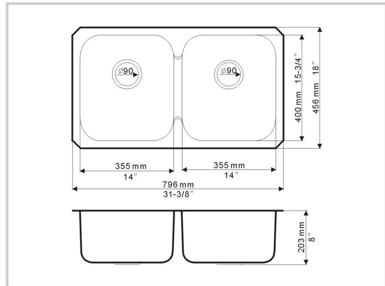
Detail Dimensions
