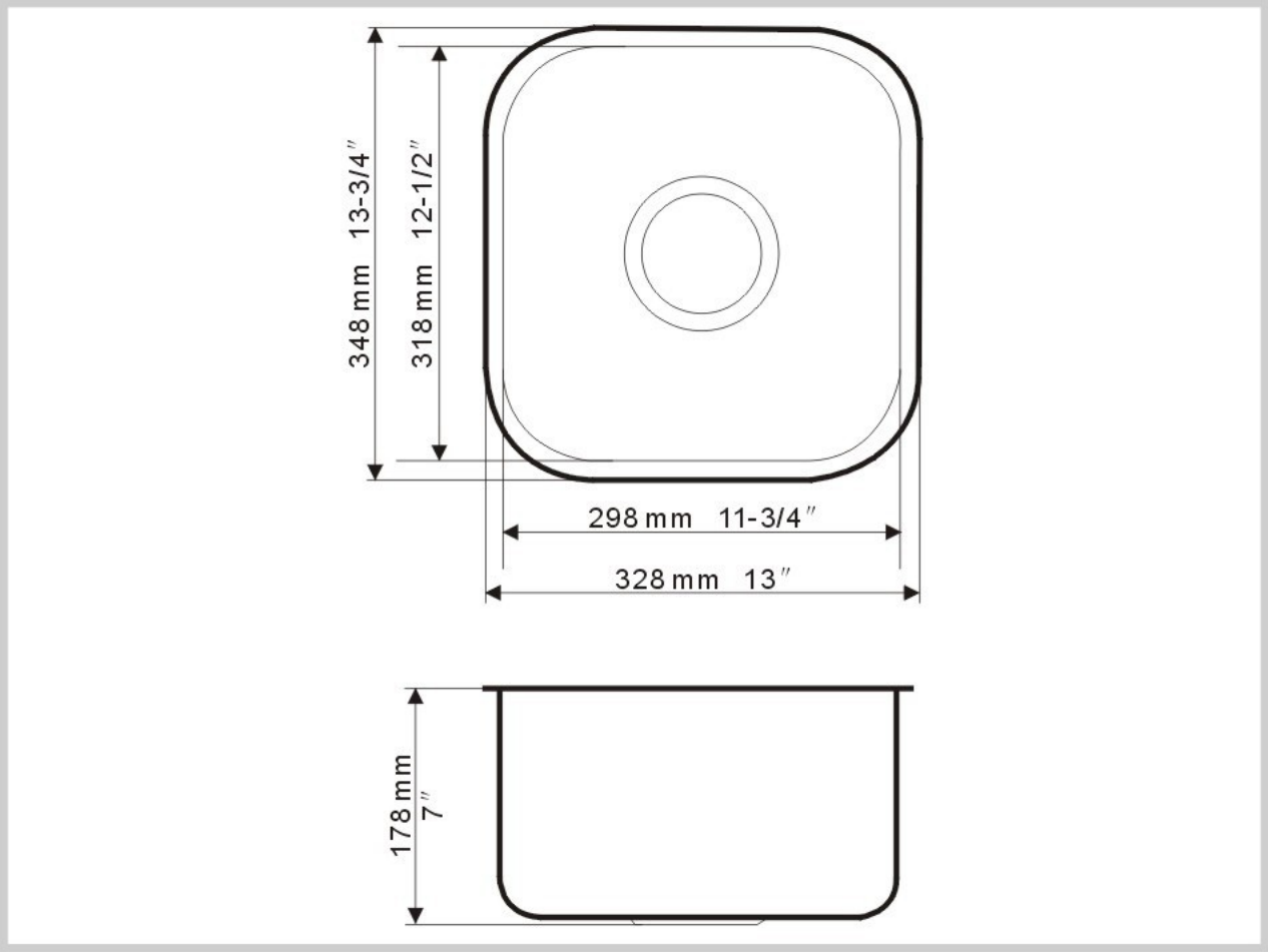
Detail Dimensions
