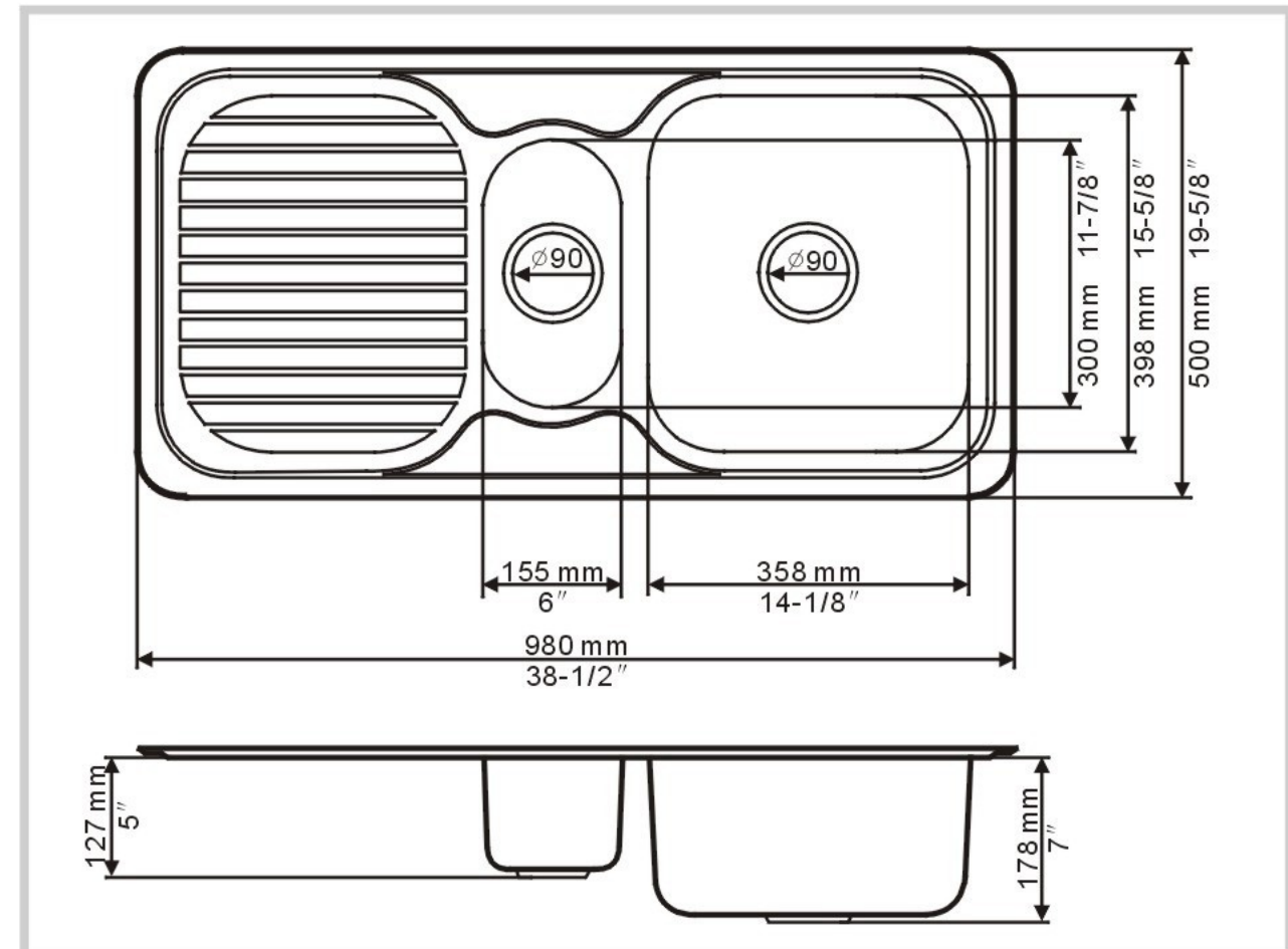
Detail Dimensions
