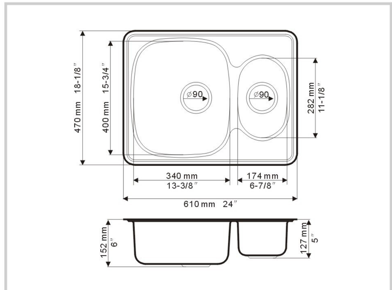
Detail Dimensions
