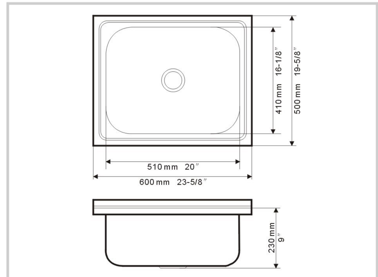
Detail Dimensions
