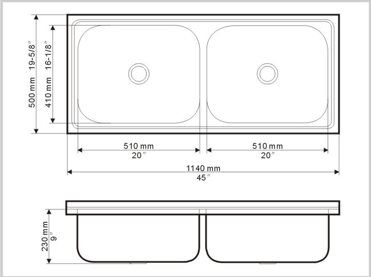
Detail Dimensions
