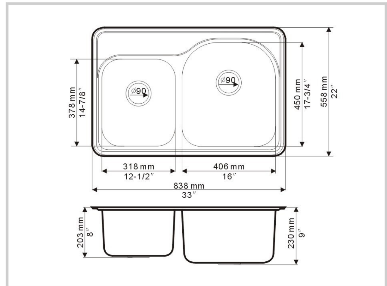
Detail Dimensions
