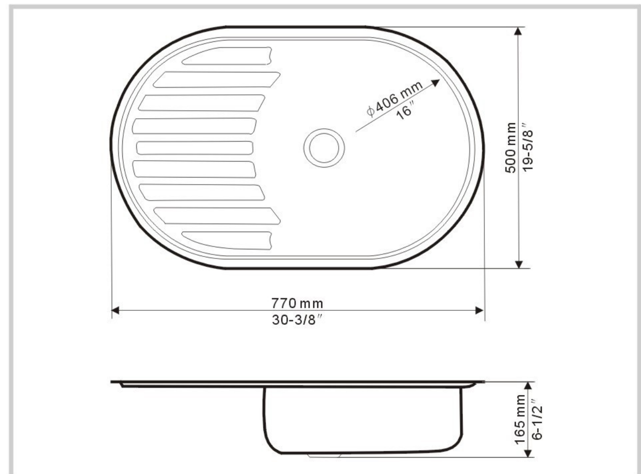
Detail Dimensions
