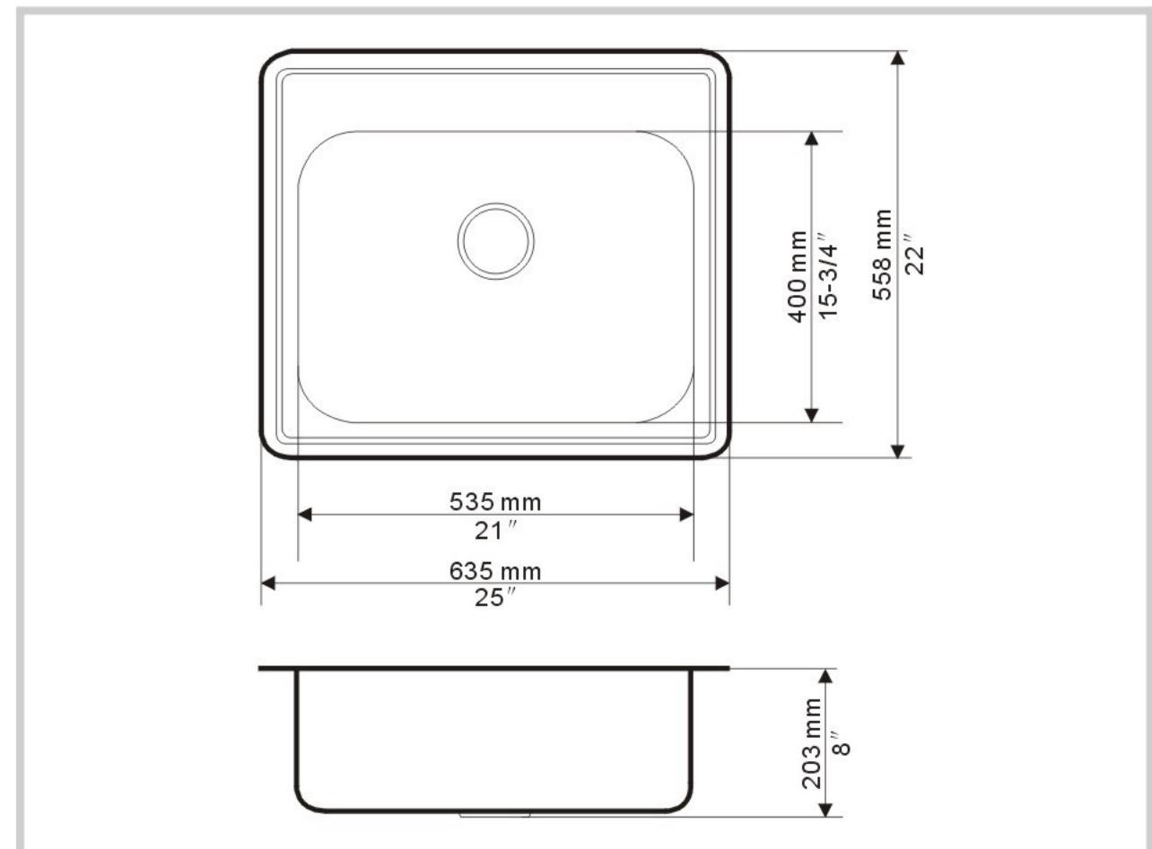
Detail Dimensions
