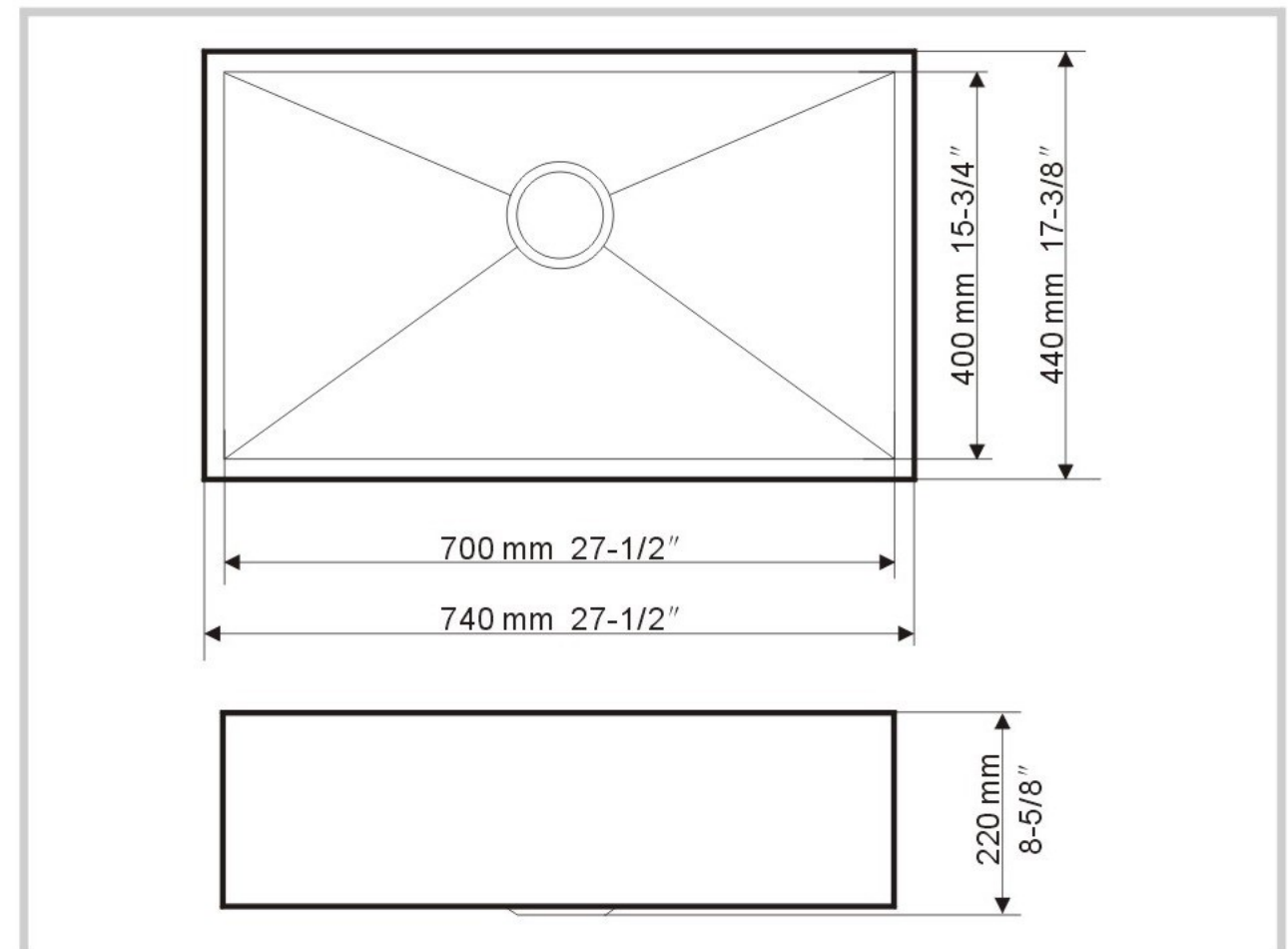
Detail Dimensions
