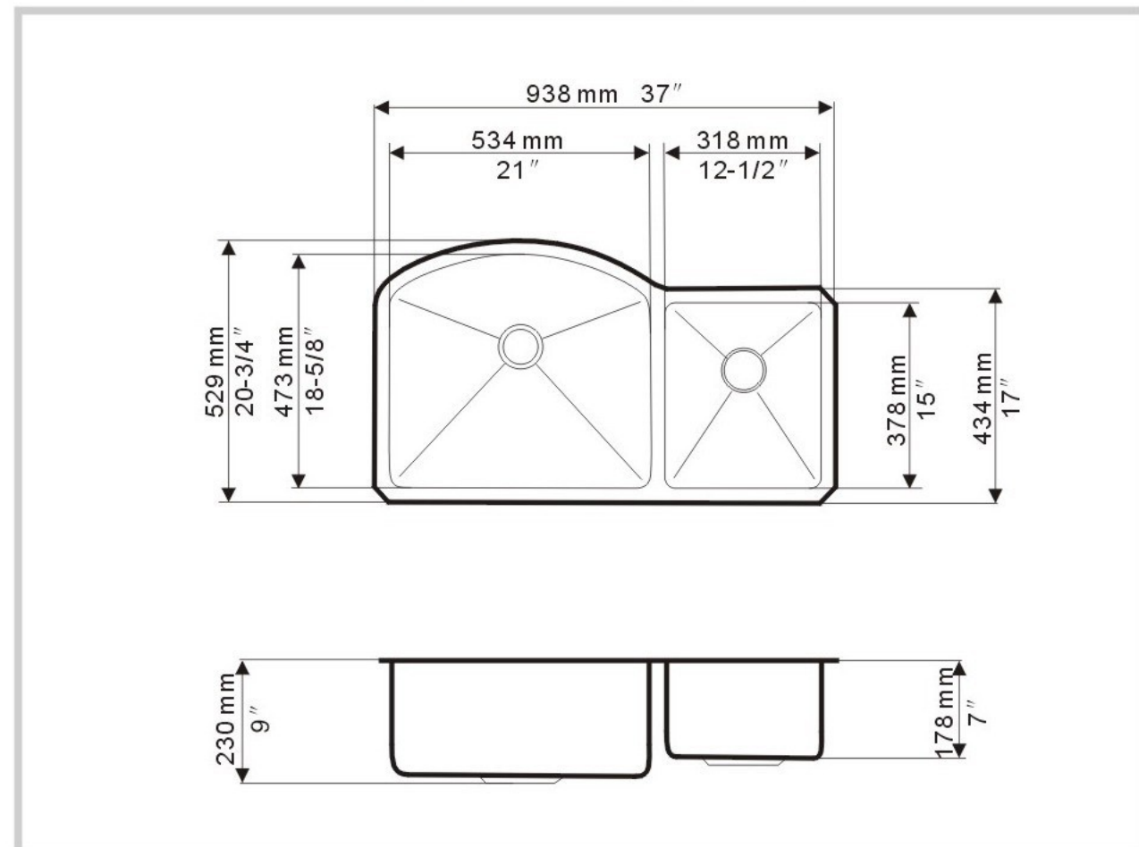
Detail Dimensions
