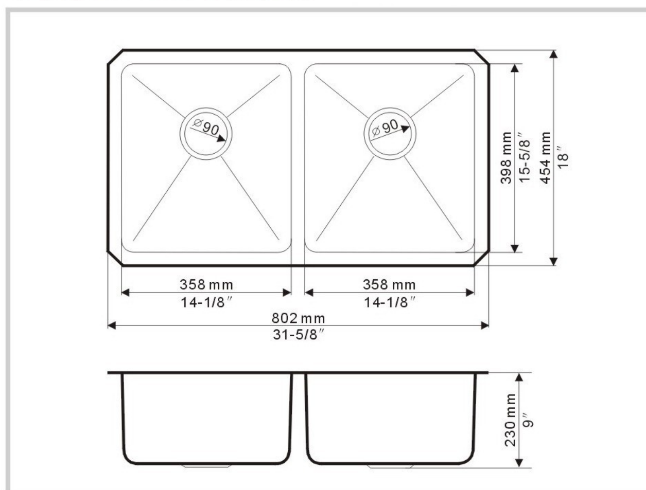
Detail Dimensions
