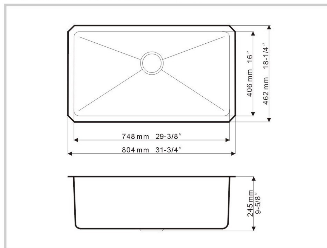
Detail Dimensions
