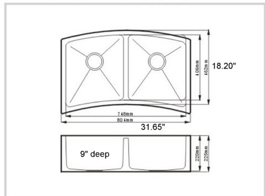
Detail Dimensions
